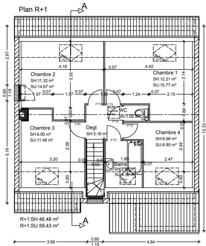
PLAN ETAGE COTE/SURFACE
